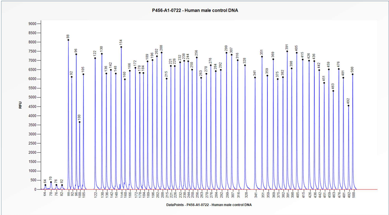
Figure 1. Capillary electrophoresis pattern from a sample of approximately 50 ng human male control DNA analysed with SALSA MLPA Probemix P456 EVC EVC2 (A1-0722).
