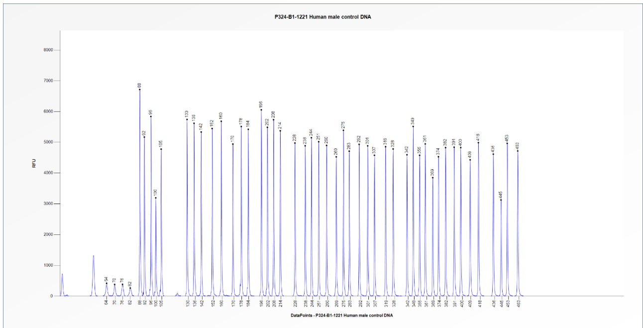
Figure 1. Capillary electrophoresis pattern from a sample of approximately 50 ng human male control DNA analysed with SALSA MLPA Probemix P324 22q11 (B1-1221).
