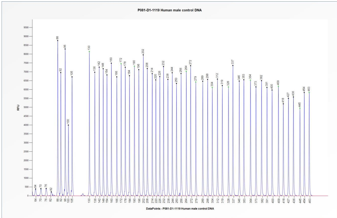
Figure 1. Capillary electrophoresis pattern from a sample of approximately 50 ng human male control DNA analysed with SALSA MLPA Probemix P081 NF1 mix 1 (D1-1119).
