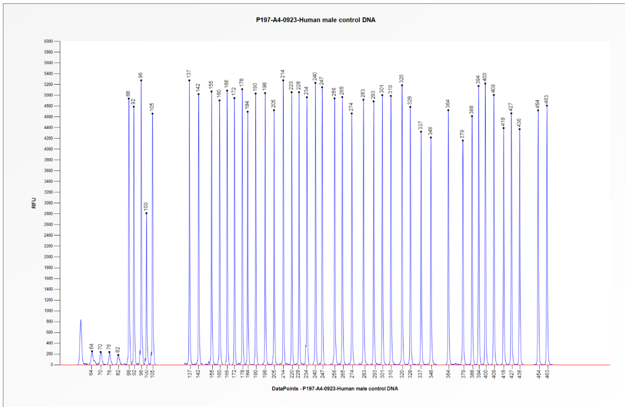
Figure 1. Capillary electrophoresis pattern from a sample of approximately 50 ng human male control DNA analysed with SALSA MLPA Probemix P197 KCNQ3 (A4-0923).
