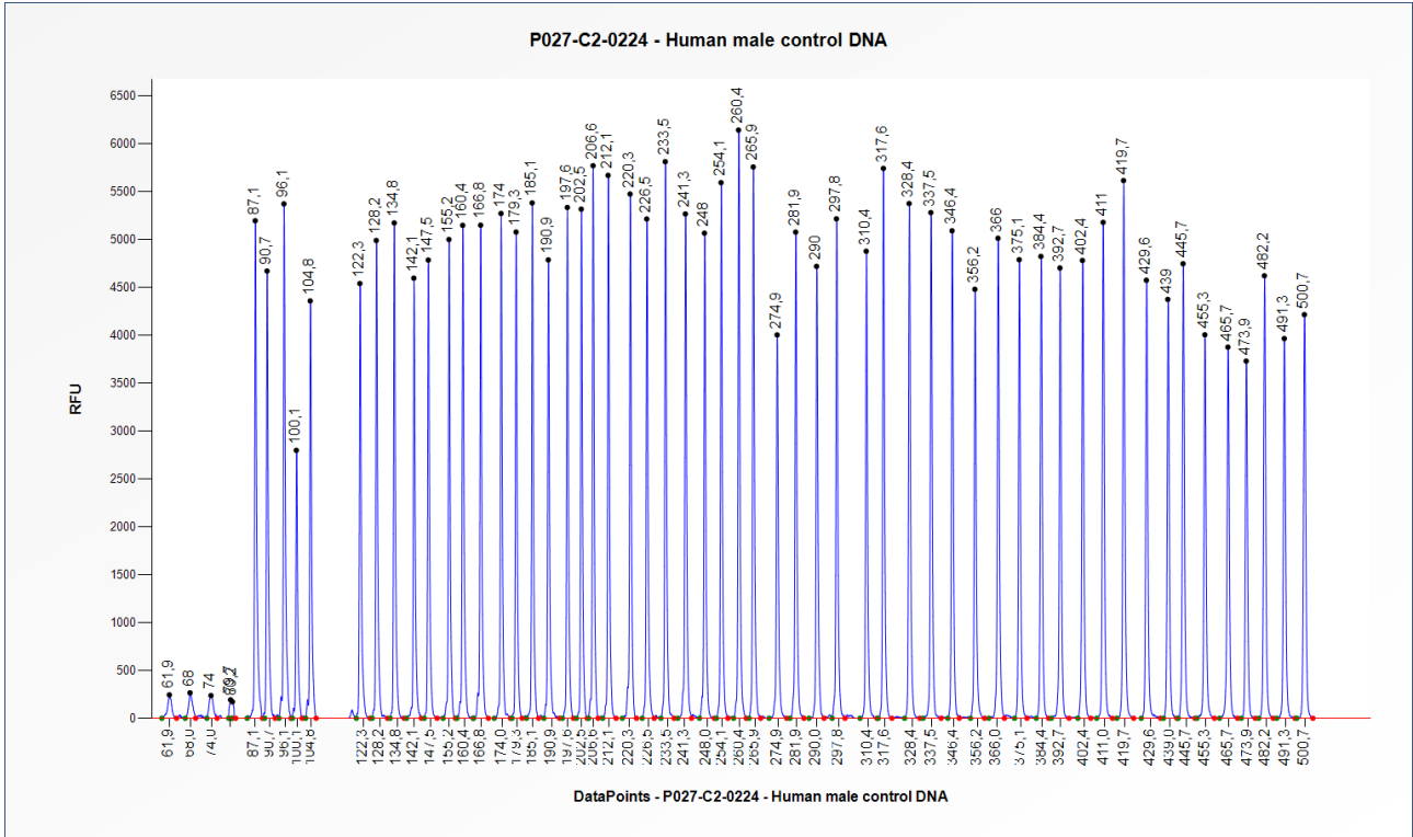
Figure 1. Capillary electrophoresis pattern from a sample of approximately 50 ng human male control DNA analysed with SALSA MLPA Probemix P027 Uveal melanoma (C2-0224).
