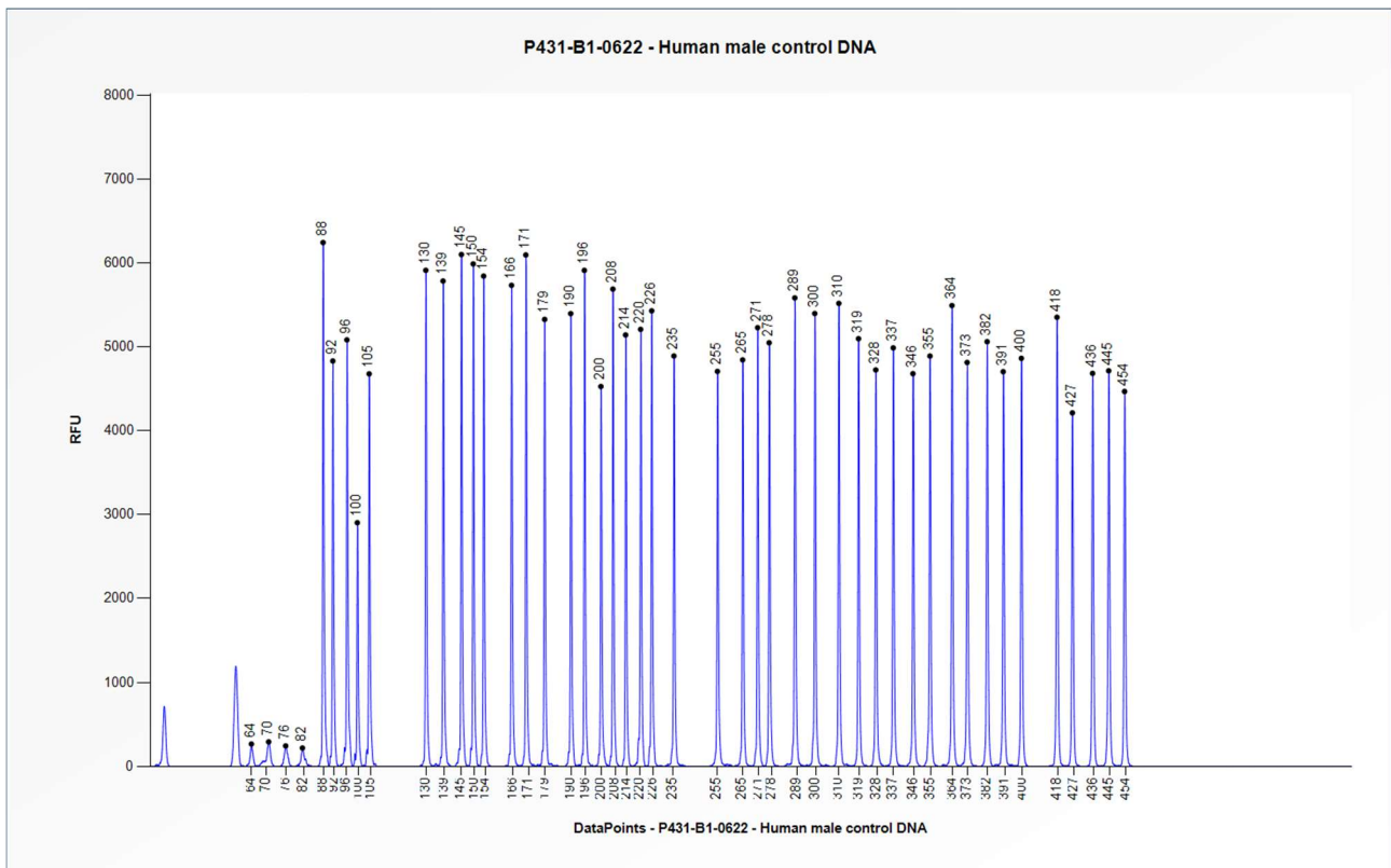
Figure 1. Capillary electrophoresis pattern from a sample of approximately 50 ng human male control DNA analysed with SALSA MLPA Probemix P431 FOXF1 (B1-0622).
