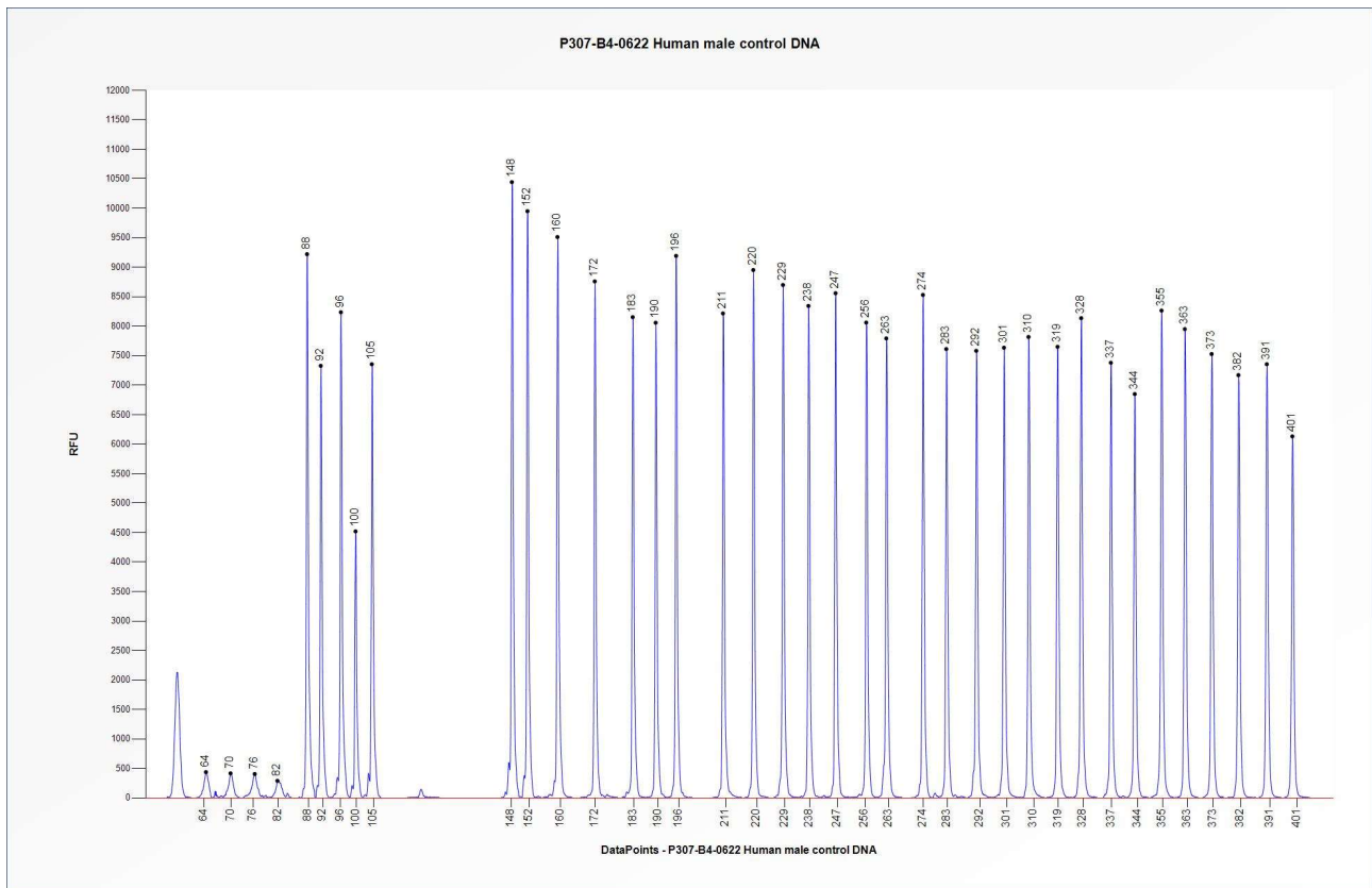
Figure 1. Capillary electrophoresis pattern from a sample of approximately 50 ng human male control DNA analysed with SALSA MLPA Probemix P307 SEPT9 (B4-0622).
