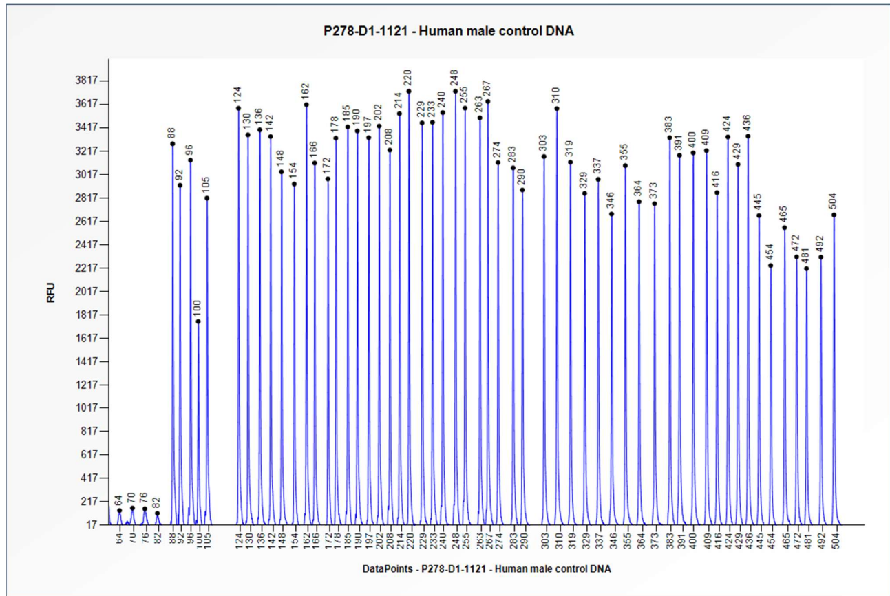
Figure 1. Capillary electrophoresis pattern from a sample of approximately 50 ng human male control DNA analysed with SALSA MLPA Probemix P278 PCCA-PCCB (D1-1121).
