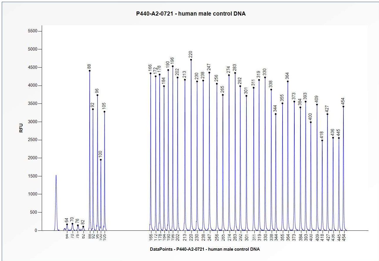
Figure 1. Capillary electrophoresis pattern from a sample of approximately 50 ng human male control DNA analysed with SALSA MLPA Probemix P440 F10 + F11 (A2-0721).
