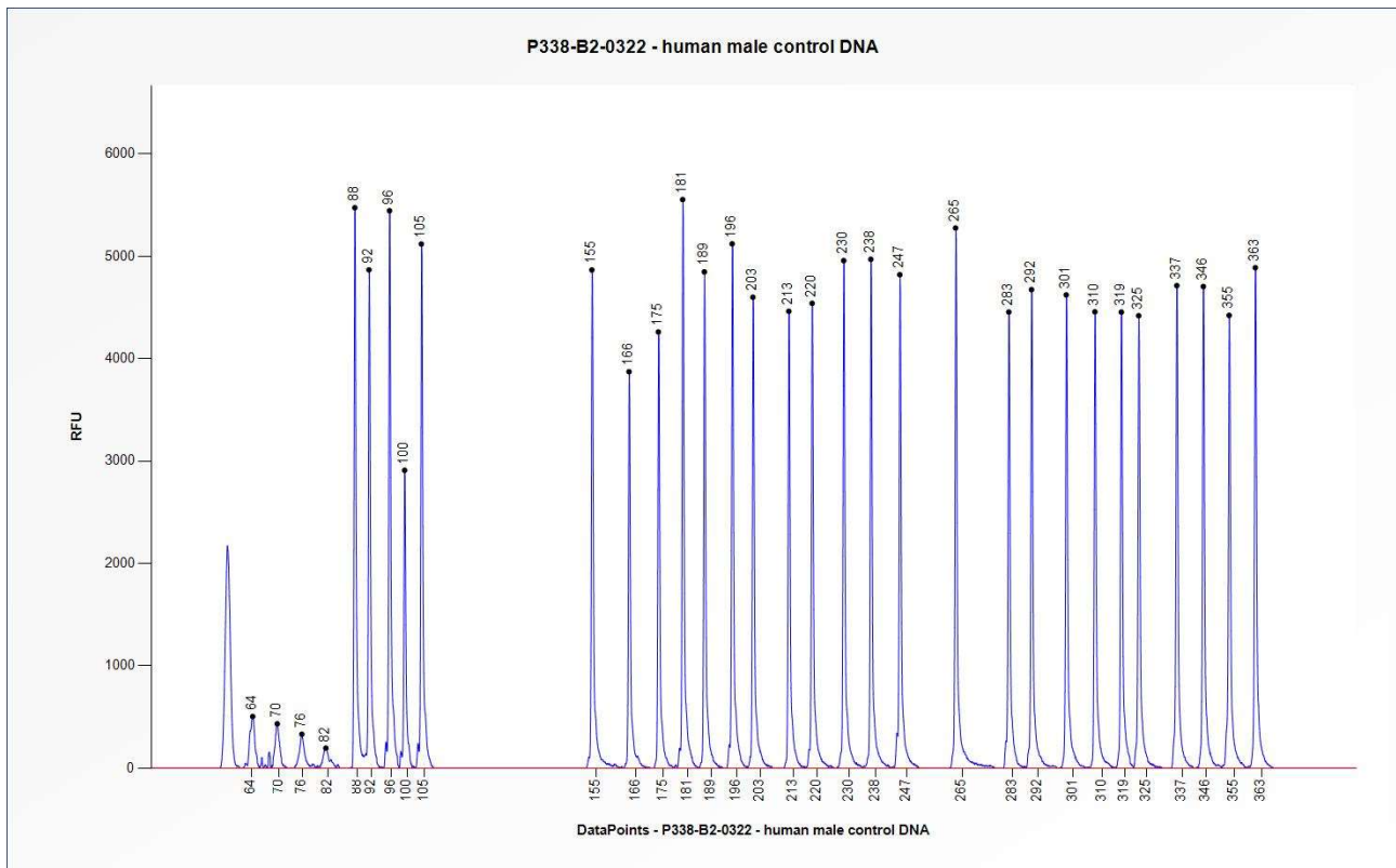
Figure 1. Capillary electrophoresis pattern from a sample of approximately 50 ng human male control DNA analysed with SALSA MLPA Probemix P338 GBA (B2-0322).
