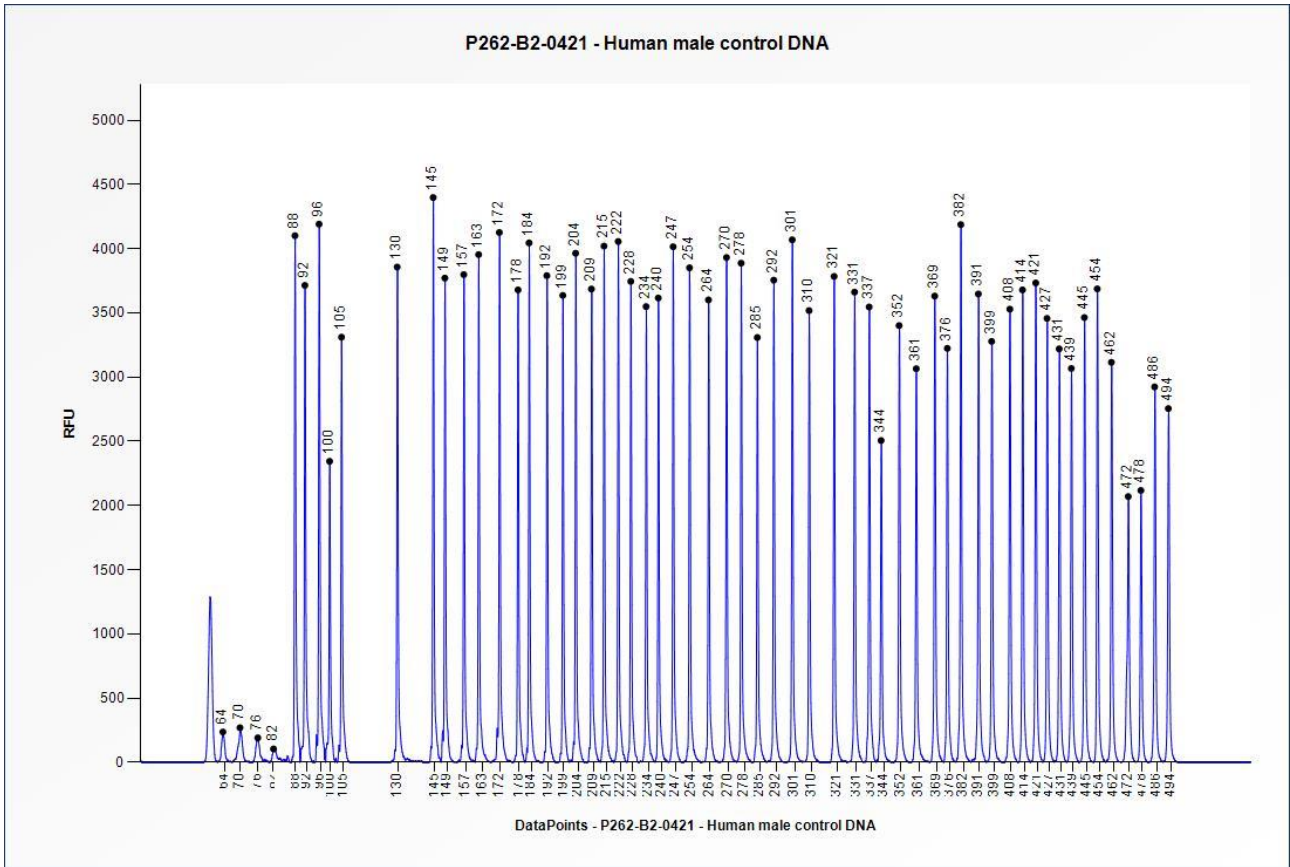
Figure 1. Capillary electrophoresis pattern from a sample of approximately 50 ng human male control DNA analysed with SALSA MLPA Probemix P262 GHI (B2-0421).
