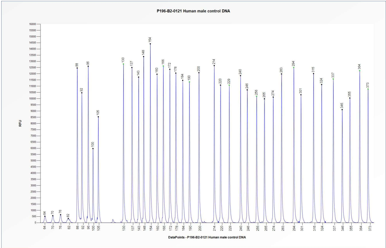
Figure 1. Capillary electrophoresis pattern from a sample of approximately 50 ng human male control DNA analysed with SALSA MLPA Probemix P196 TNNT2-BAG3 (B2-0121).
