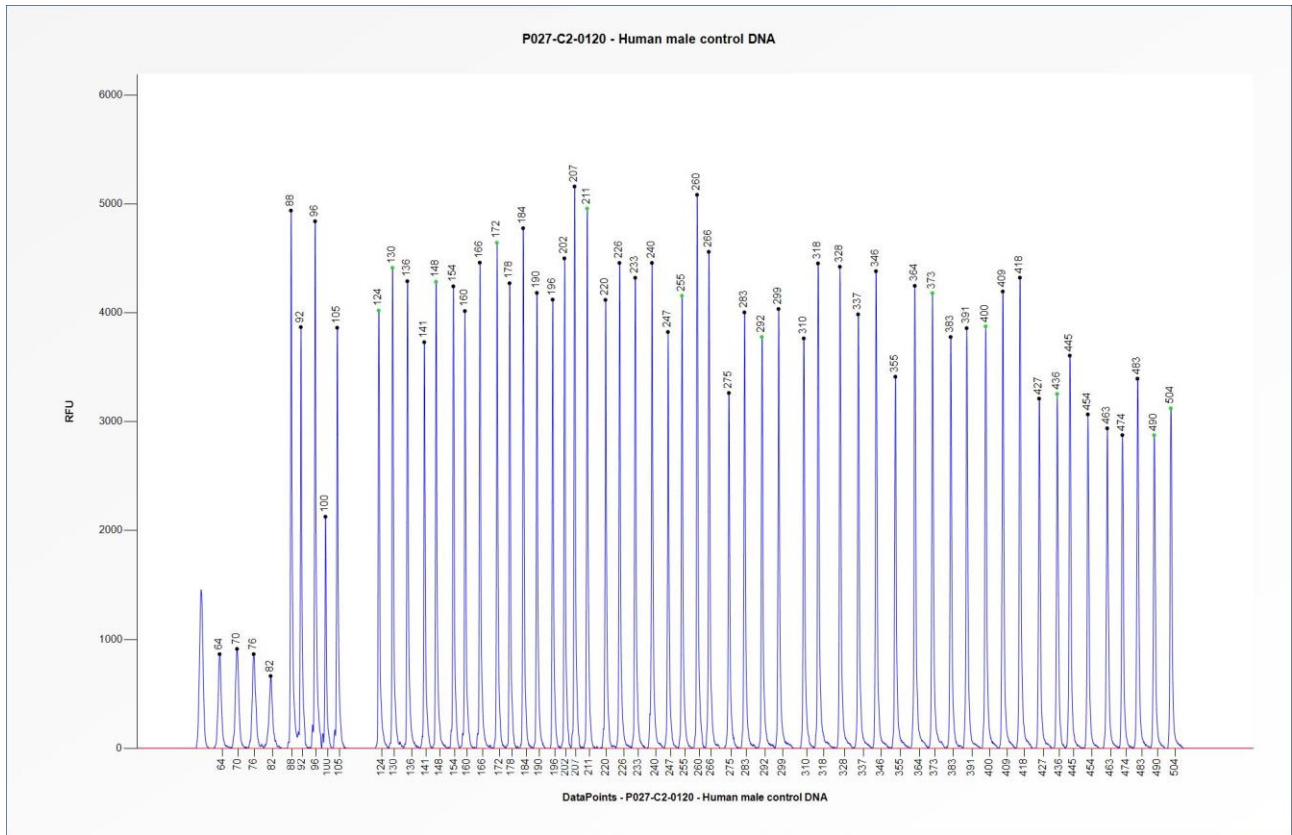
Figure 1. Capillary electrophoresis pattern from a sample of approximately 50 ng human male control DNA analysed with SALSA MLPA Probemix P027 Uveal melanoma (C2-0120).
