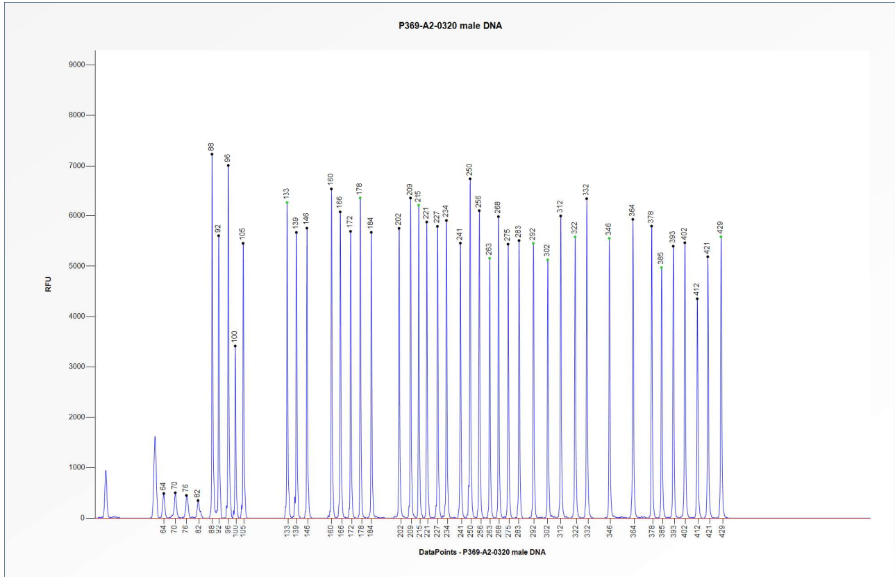
Figure 1. Capillary electrophoresis pattern from a sample of approximately 50 ng human male control DNA analysed with SALSA MLPA Probemix P369 Smith-Magenis Syndrome (A2-0320).
