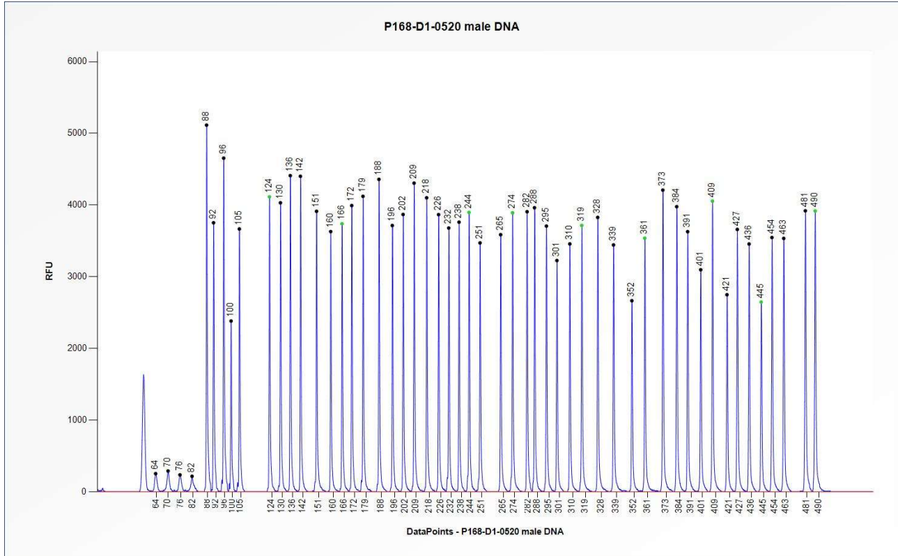
Figure 1. Capillary electrophoresis pattern from a sample of approximately 50 ng human male control DNA analysed with SALSA MLPA Probemix P168 ARVC-CPK2 (D1-0520).
