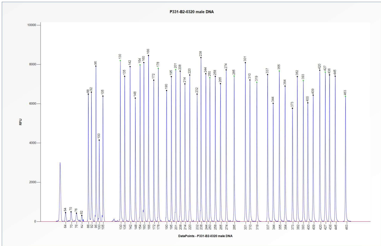
Figure 1. Capillary electrophoresis pattern from a sample of approximately 50 ng human male control DNA analysed with SALSA MLPA Probemix P331 COL5A1 MIX-1 (B2-0320).
