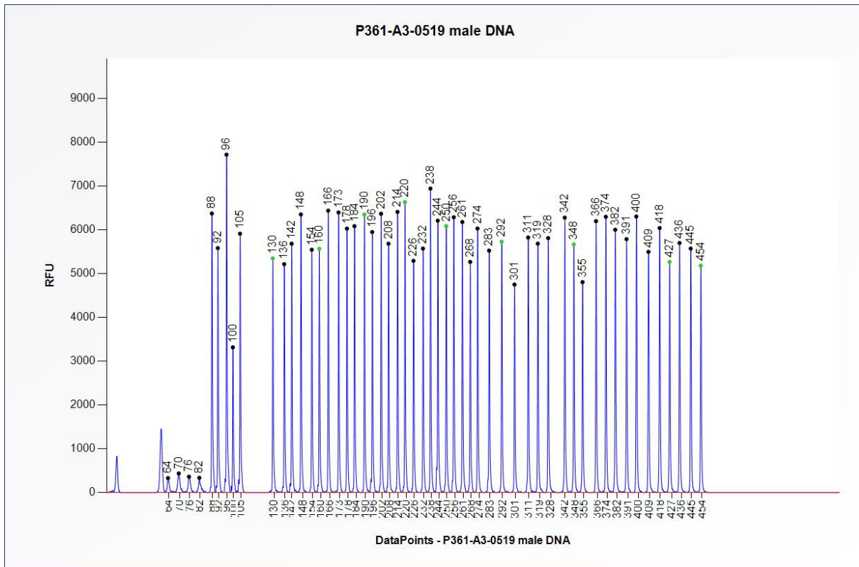
Figure 1. Capillary electrophoresis pattern from a sample of approximately 50 ng human male control DNA analysed with SALSA MLPA Probemix P361 USH2A mix 1 (A3-0519).
